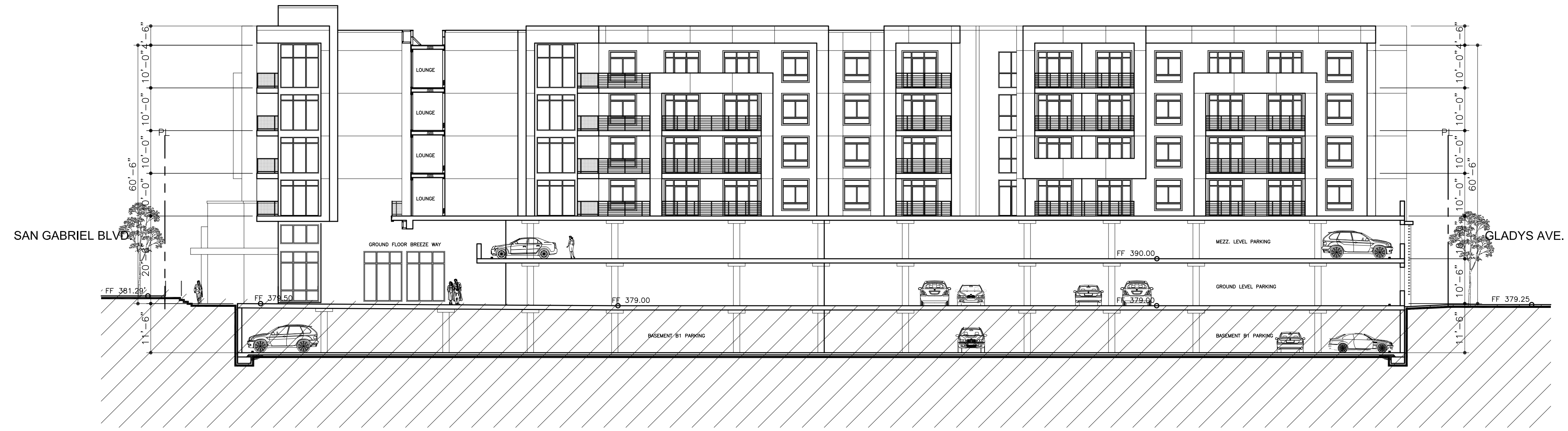
700 PLAZA SECTION 6
