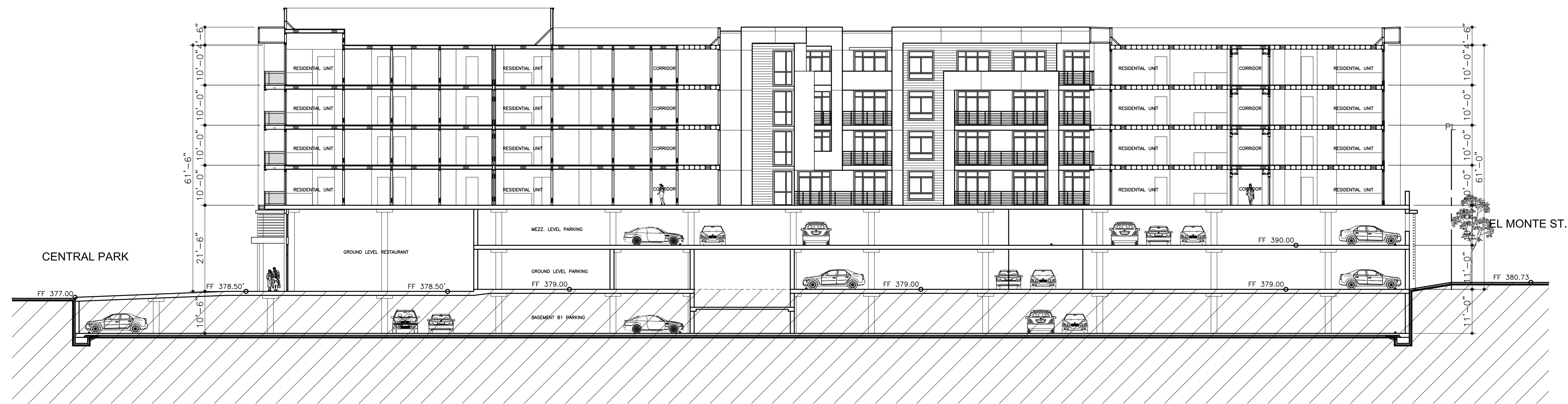
700 PLAZA SECTION 4
