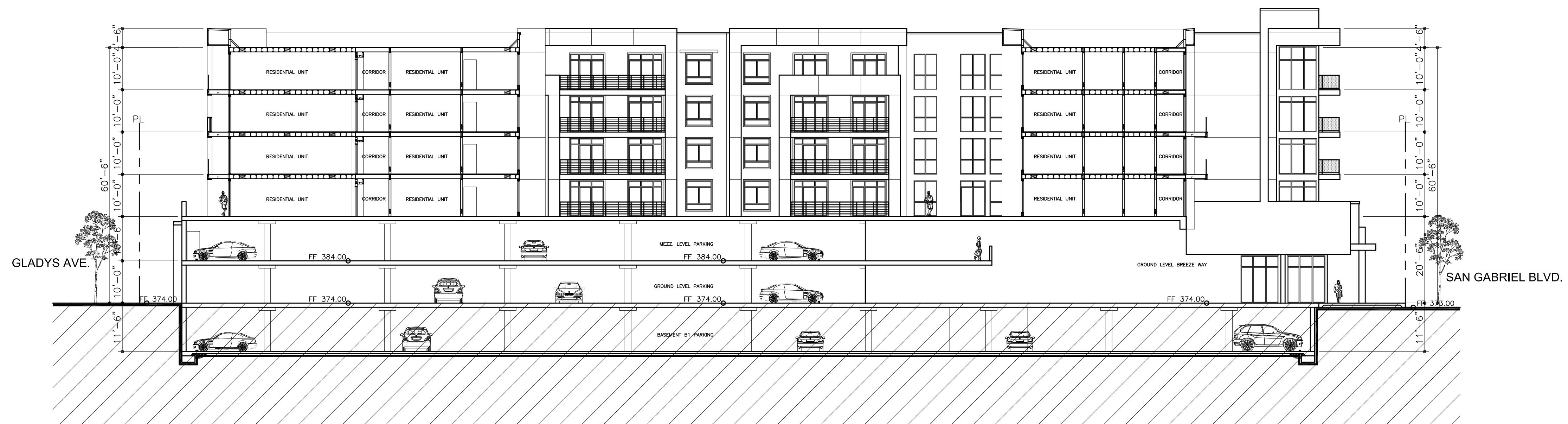
800 PLAZA SECTION 7
