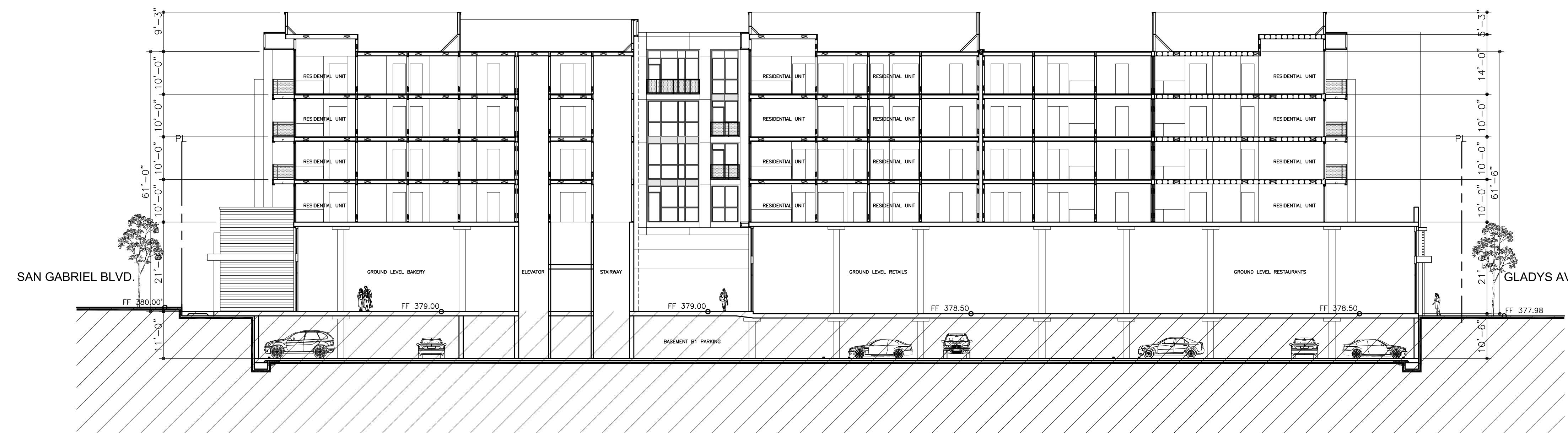
700 PLAZA SECTION 8
