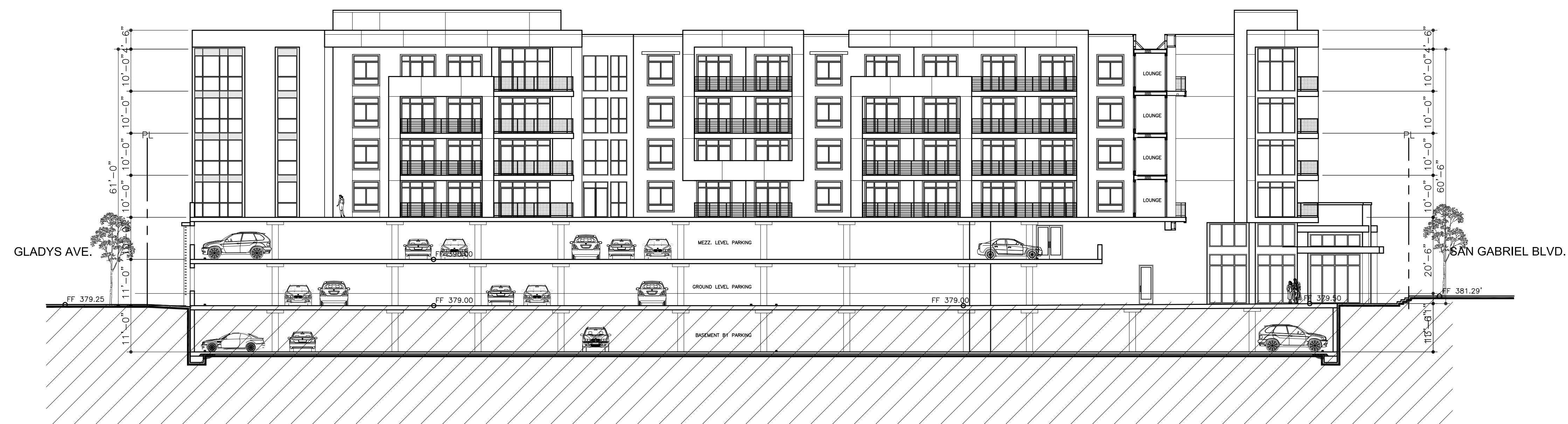
700 PLAZA SECTION 7
